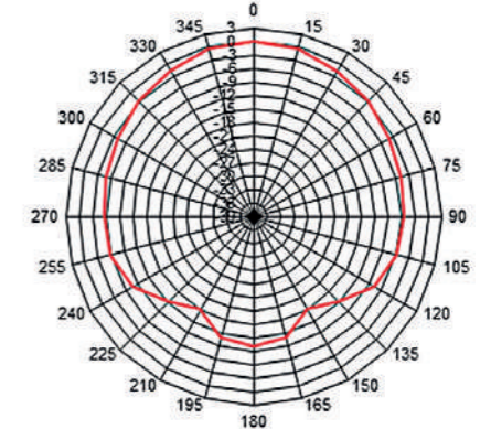
Directivity @ 1kHz
