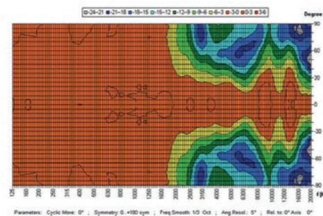
Polar diagrams
