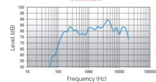
Bandwidth
