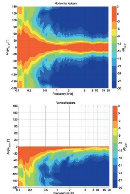
Polar diagrams
