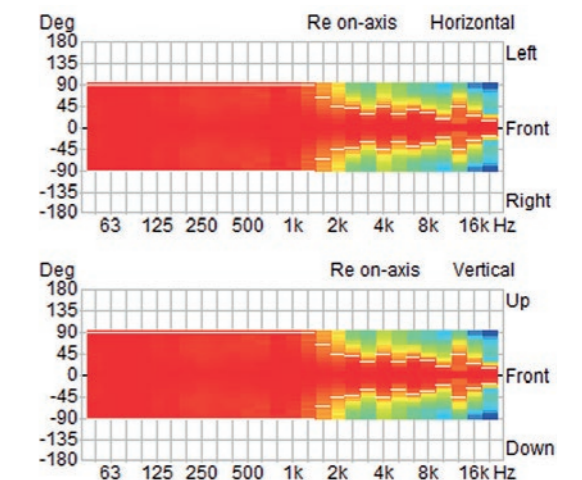
Polar diagrams
