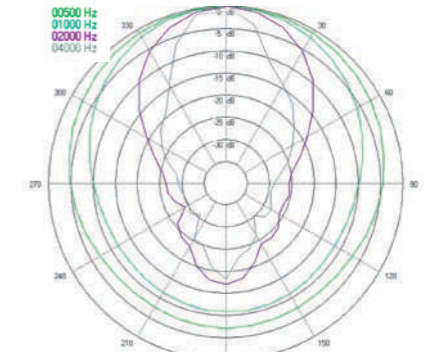
Directivity
